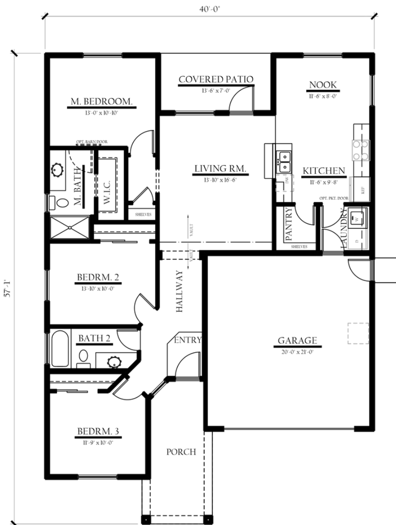
1340 Floorplan
