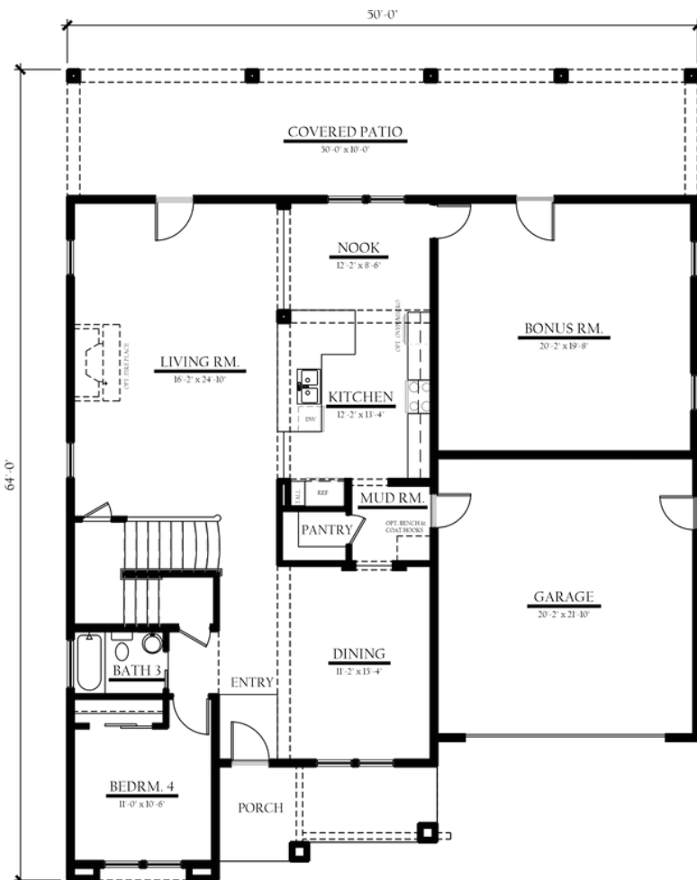
3155 Lower Floorplan
